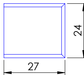
Deckel/Boden 4x
